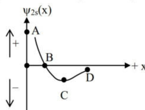
Figure 2. wave function for 2s orbital
