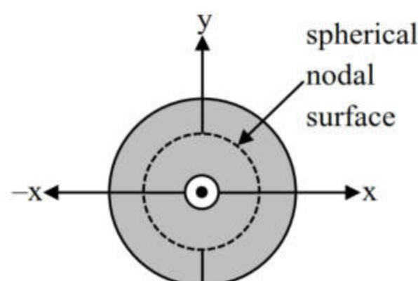
Figure 1. electron probability density for 2s orbital
