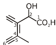
3-ethynyl-2-hydroxy-4-methylhex-3-en-5-ynoic acid
