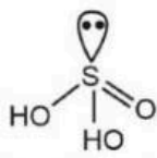
Sulphurous acid ( \text{H}_2\text{SO}_3 )
