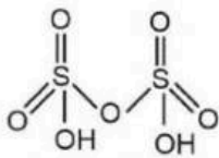
Pyrosulphuric acid ( \text{H}_2\text{S}_2\text{O}_7 )
