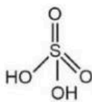
Sulphuric acid ( \text{H}_2\text{SO}_4 )
