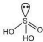
Sulphurous acid ( \text{H}_2\text{SO}_3 )
