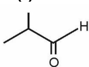
2-Methylpropanal
