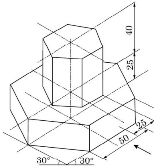
Isometric Projection
